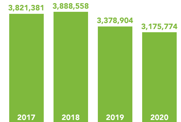
Inter-dealer trades, 2017–2020
