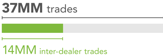
Inter-dealer trades, 2017–2020
