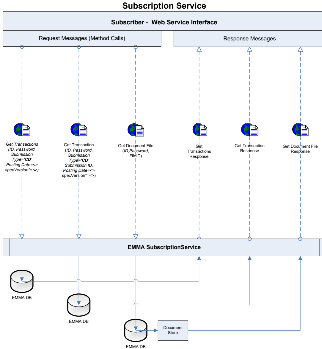
Figure 1: Message Processing Overview for the EMMA Subscription Web Service Interface
